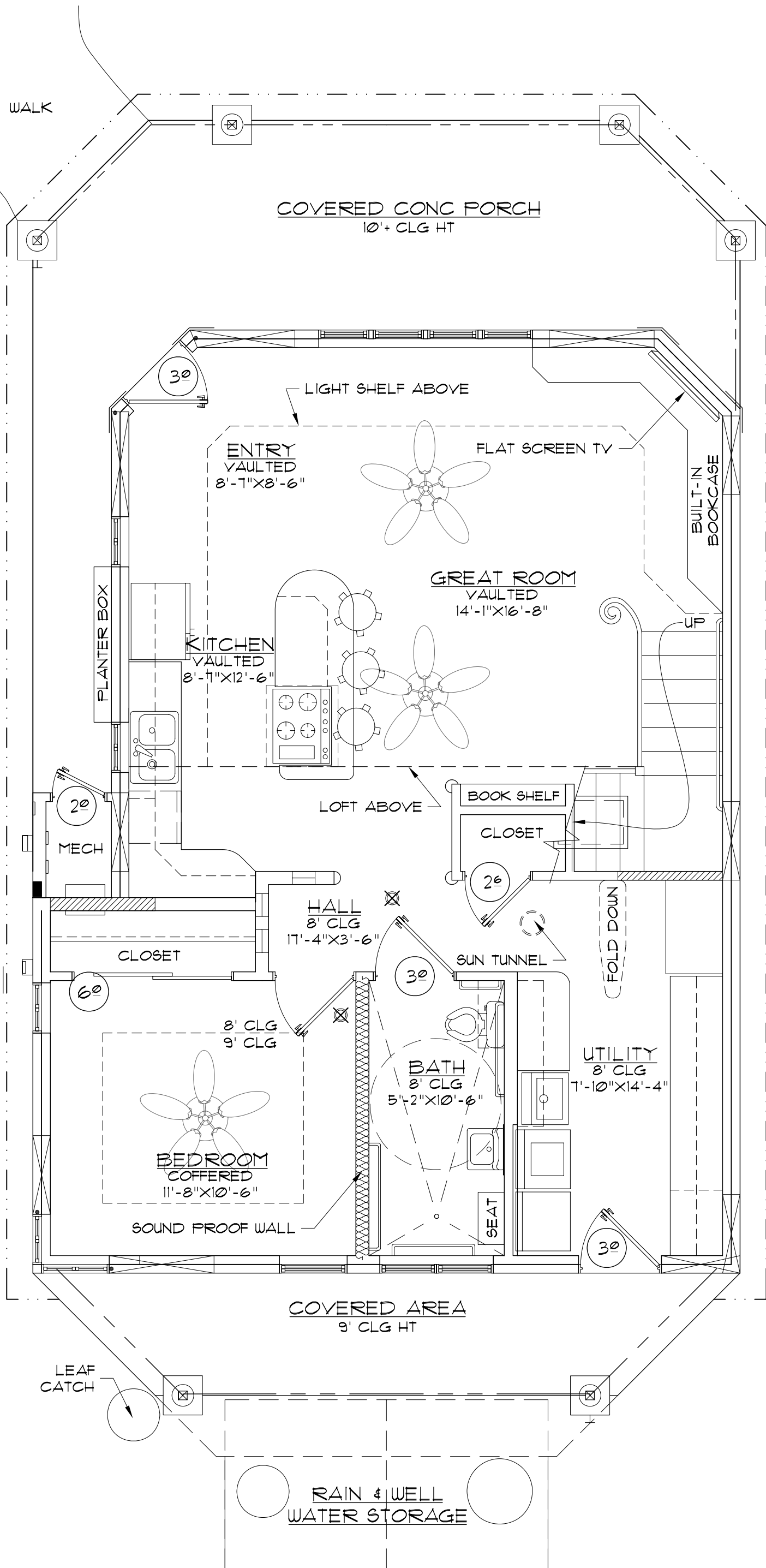
MAIN FLOOR PLAN
